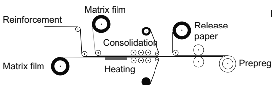
Figure 3.2 Manufacturing methods, left: hot melt process; right: solvent process
