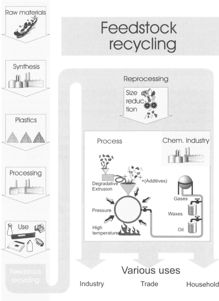
Figure 20-4 Raw material recycling using degradative extrusion
