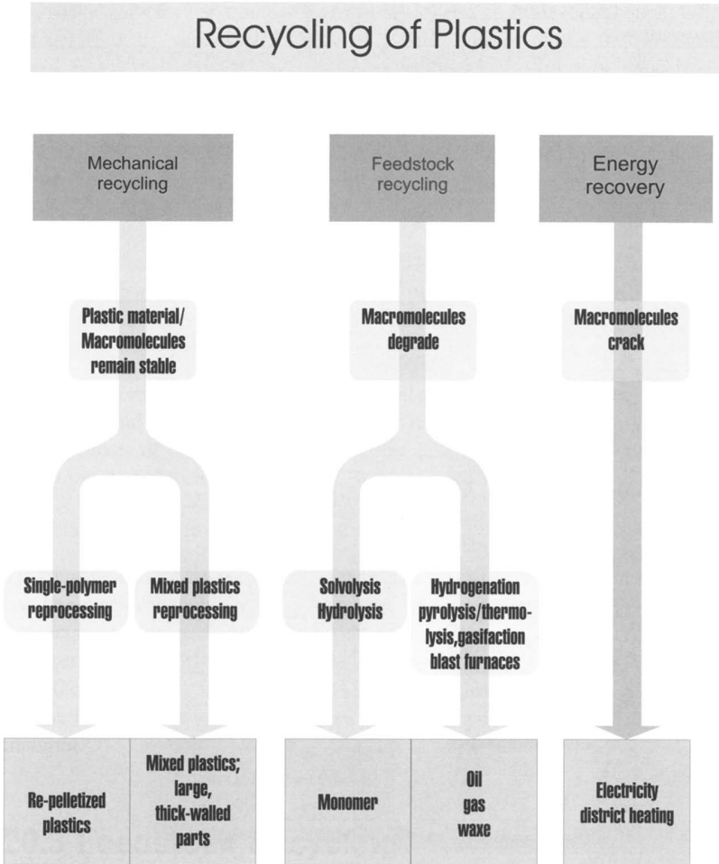
Figure 20-1 Recycling cycles
